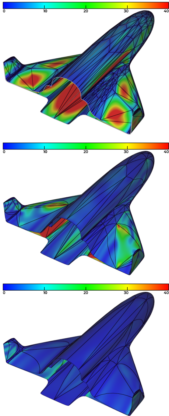
Figure 7: P^1 (top), P^2 (middle) and P^3 (bottom) point-wise distance to the shuttle geometry.
