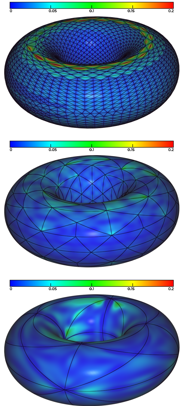
Figure 5: P^1 (top), P^2 (middle) and P^3 (bottom) point-wise distance to the torus geometry.
