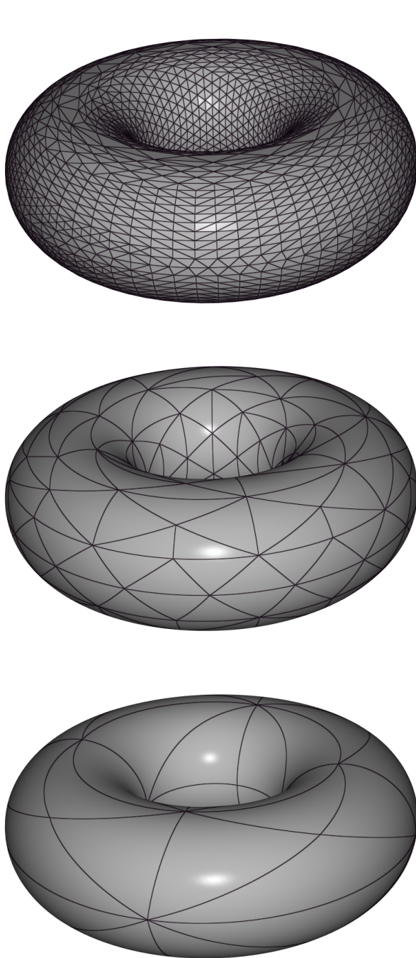
Figure 4: P^1 (top), P^2 (middle) and P^3 (bottom) meshes for the torus geometry.
